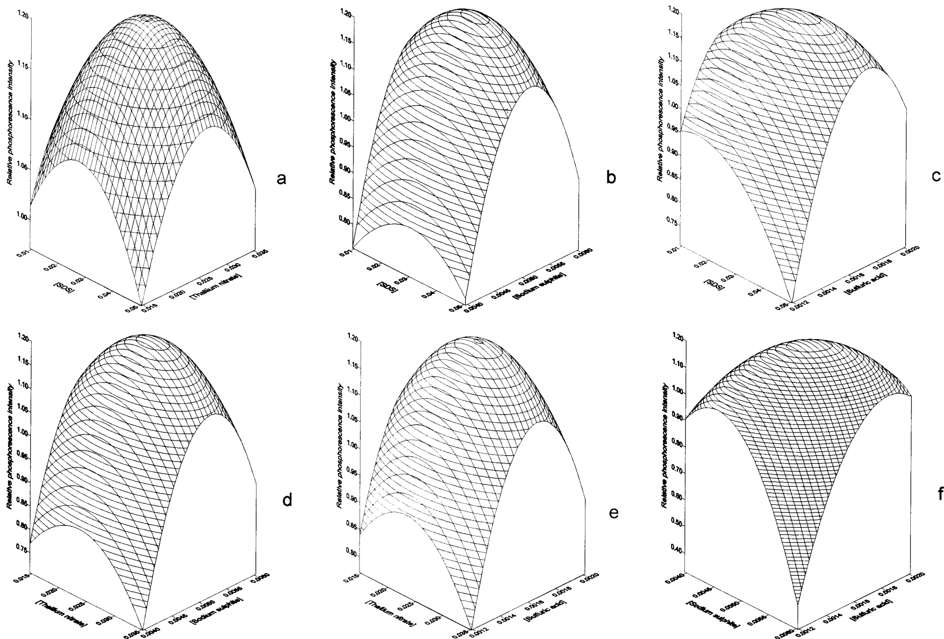
Figure 1. Surface response of NAA for (a) SDS and \text{TlNO}_3 concentrations at 5.12 \times 10^{-3} \text{ mol L}^{-1} \text{ Na}_2\text{SO}_3 and 1.63 \times 10^{-3} \text{ mol L}^{-1} \text{ H}_2\text{SO}_4 ; (b) SDS and \text{Na}_2\text{SO}_3 concentrations at 2.52 \times 10^{-2} \text{ mol L}^{-1} \text{ TlNO}_3 and 1.63 \times 10^{-3} \text{ mol L}^{-1} \text{ H}_2\text{SO}_4 ; (c) SDS and \text{H}_2\text{SO}_4 concentrations at 2.52 \times 10^{-2} \text{ mol L}^{-1} \text{ TlNO}_3 and 5.12 \times 10^{-3} \text{ mol L}^{-1} \text{ Na}_2\text{SO}_3 ; (d) \text{TlNO}_3 and \text{Na}_2\text{SO}_3 concentrations at 3.04 \times 10^{-2} \text{ mol L}^{-1} \text{ SDS} and 1.63 \times 10^{-3} \text{ mol L}^{-1} \text{ H}_2\text{SO}_4 ; (e) \text{TlNO}_3 and \text{H}_2\text{SO}_4 concentrations at 3.04 \times 10^{-2} \text{ mol L}^{-1} \text{ SDS} and 5.12 \times 10^{-3} \text{ mol L}^{-1} \text{ Na}_2\text{SO}_3 ; and (f) \text{Na}_2\text{SO}_3 and \text{H}_2\text{SO}_4 concentrations at 3.04 \times 10^{-2} \text{ mol L}^{-1} \text{ SDS} and 2.52 \times 10^{-2} \text{ mol L}^{-1} \text{ TlNO}_3 .
